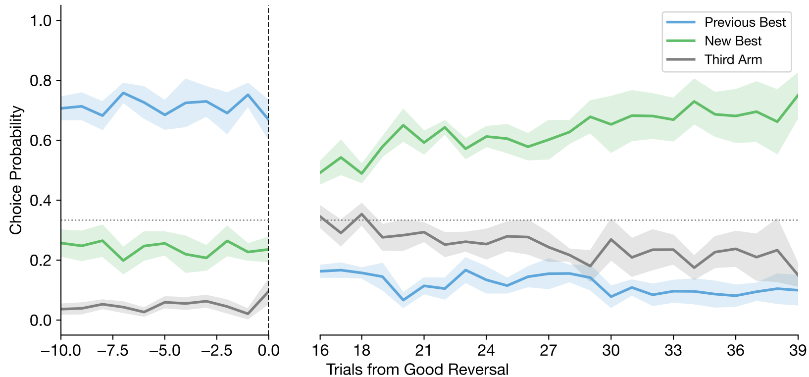
Good Reversal-Aligned Choices (mean \pm se across subjects | n=6 subjects, n=193 reversals) (Skipping first 15 trials post-reversal)
